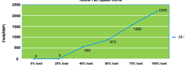
1200W Fan Speed Curve
