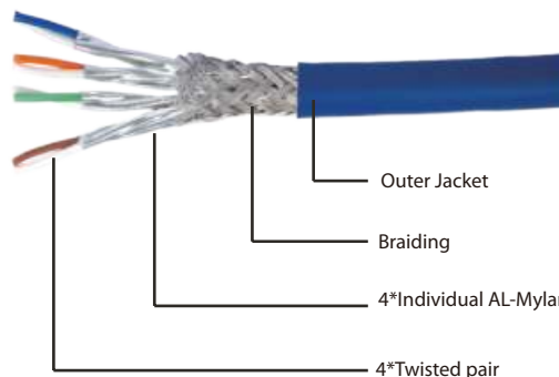
S/FTP(*PIMF): Pairs in metal foil
