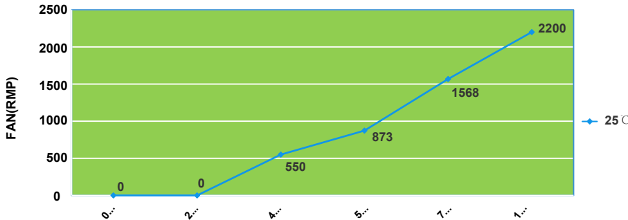
1200W Fan Speed Curve
