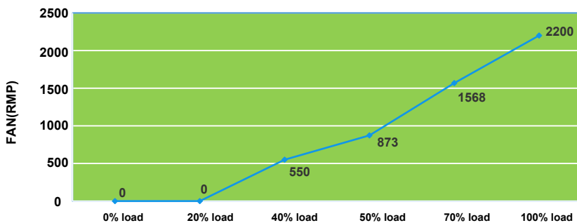
1200W Fan Speed Curve
