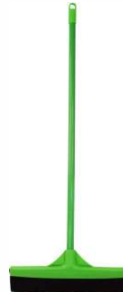
CY-308 Squeegee Description: 120cm,Φ22 Powder Coated Iron Handle With 38cm Packing: 24pcs/ctn Dimension: 121x39x16cm
